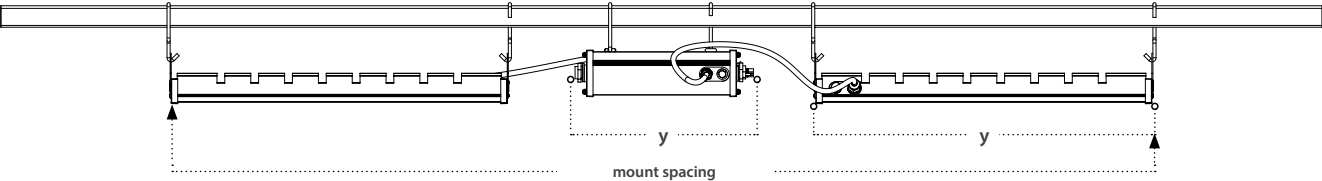
Driver Module Mounted Horizontally Below the Track
