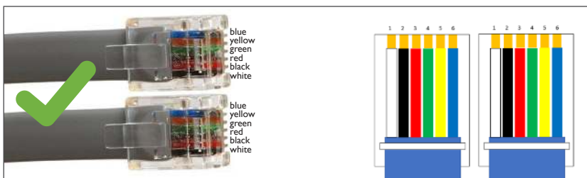
straight cable
