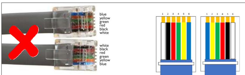
reverse cable
