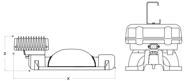
Track/Truss Bracket – End View
